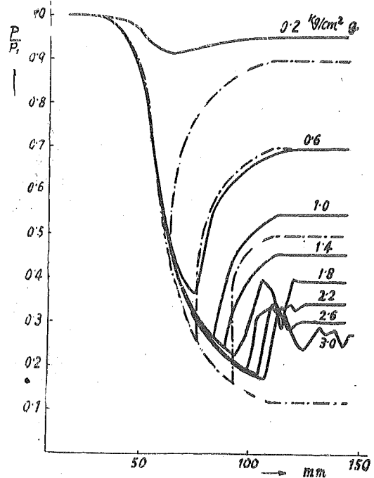
Fig. 8. Static Pressure Along the Nozzle Axis
