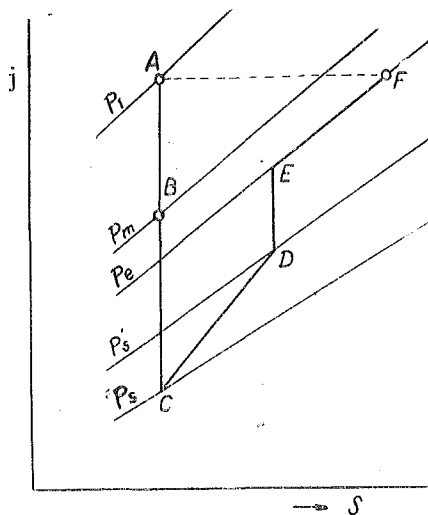
Fig. 2. Over-expansion in i, s -Diagram
