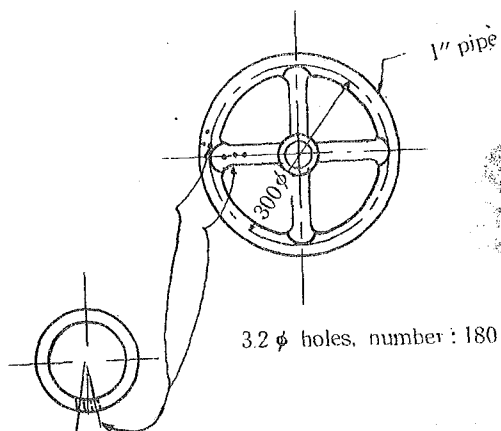
Fig. 3. Water Distributor
