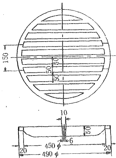
Fig. 4. Packing Support
