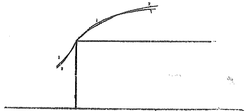
Fig. 2B. Examples of the boundary of turbulent area.
