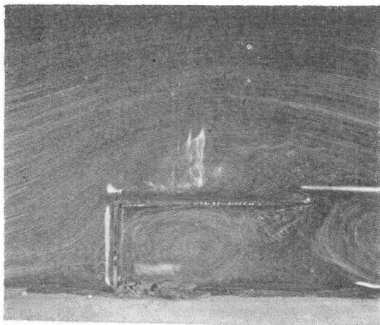
Fig. 2. A. The path lines of free surface
