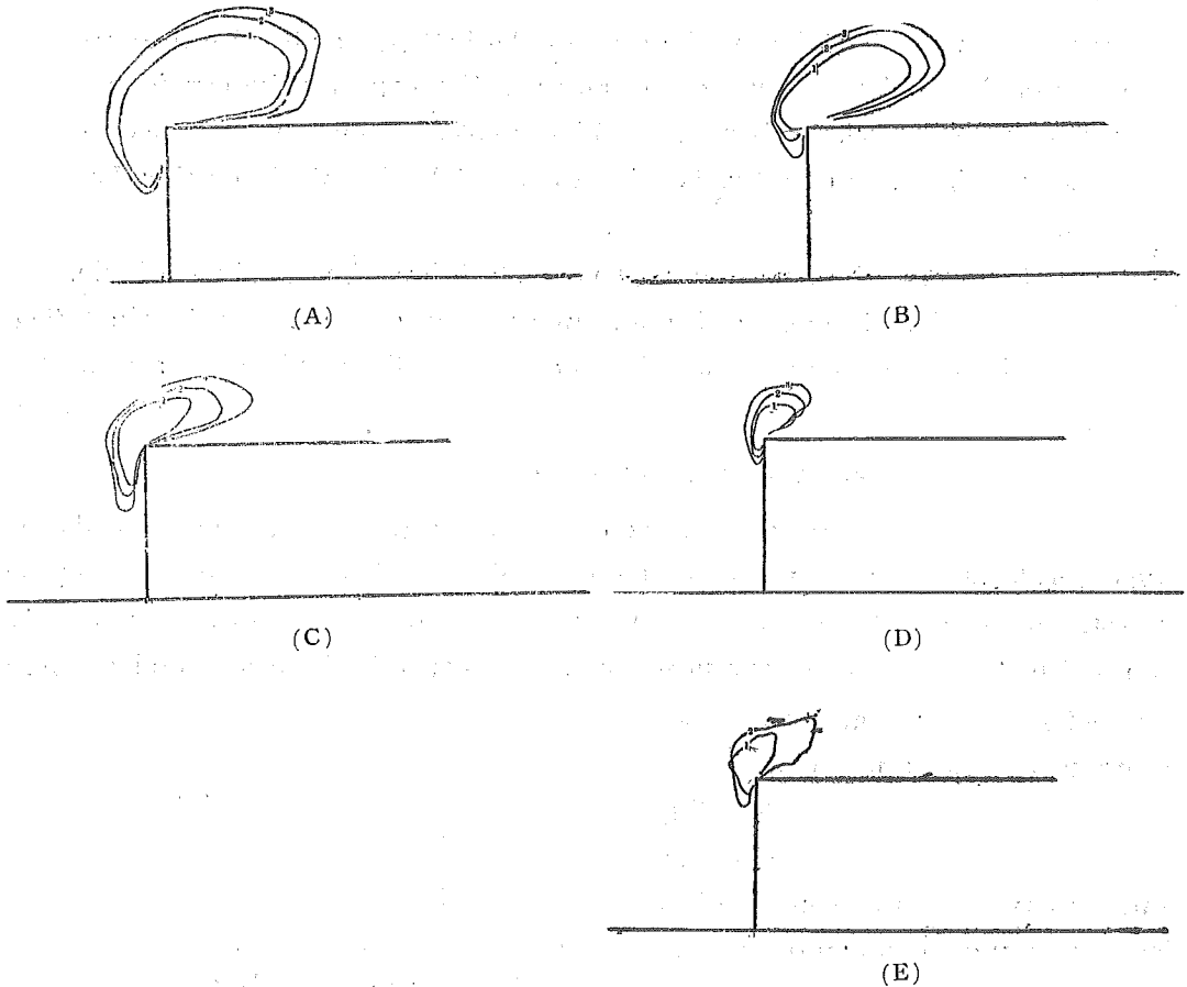
Fig. 4. The contour lines of the movement of the sand.
