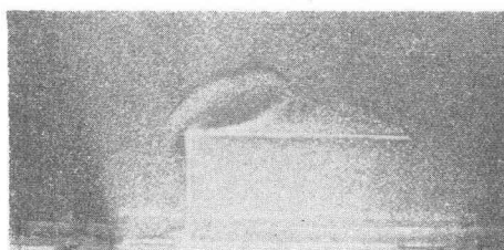
Fig. 5. A photograph of contour line formed by the movement of the sand. This state is the same as Fig. 3A.
