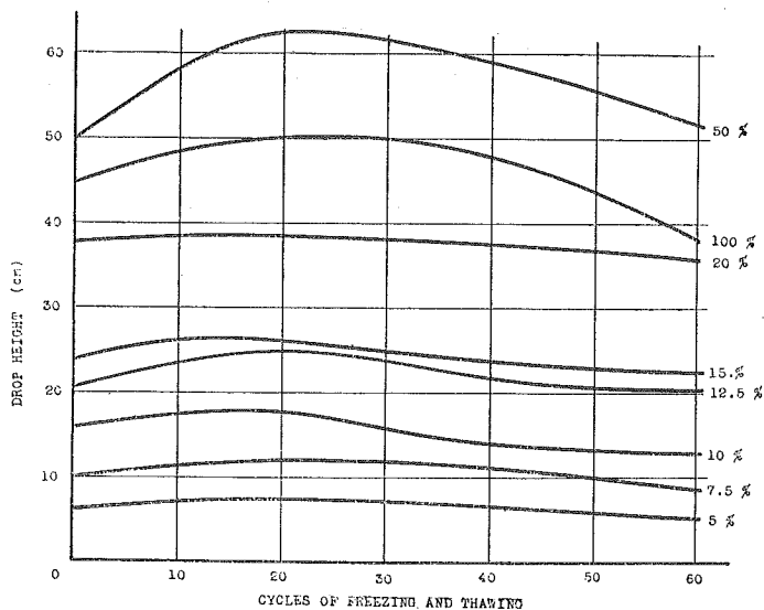
Fig. 41 Relation between toughenss of Trinidad Lake asphalt mortar and cycles of freezing and thawing. (by Page impact testing machine)
