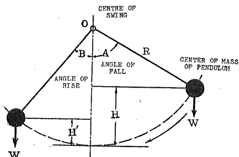
Fig. 1 Space relation for pendulum machine.
