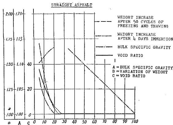
Fig. 43 Relation of bulk specific gravity, variation of weight, void ratio and asphalt content.
