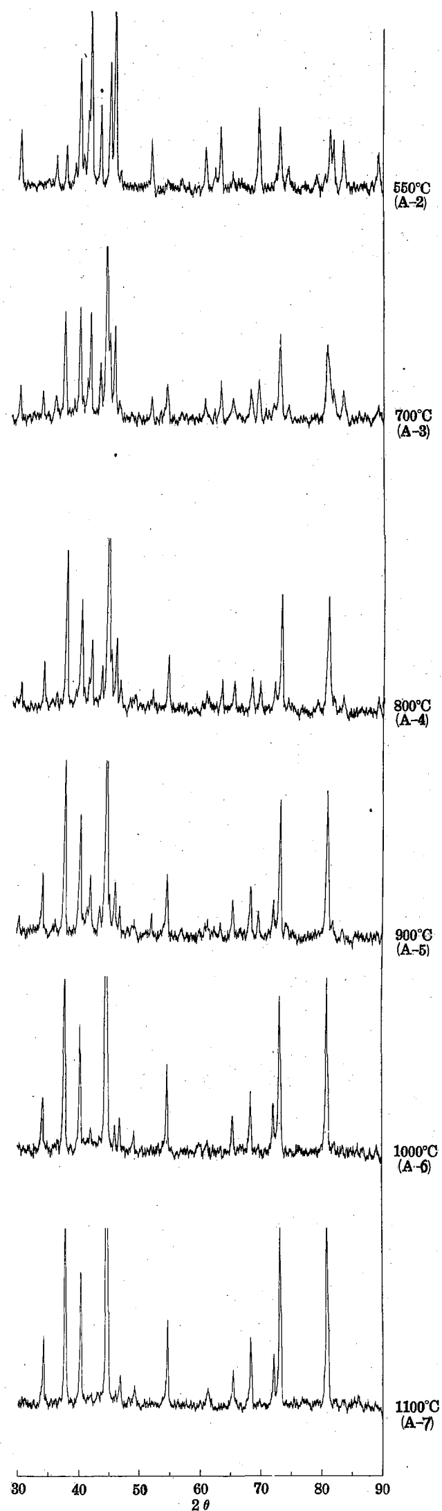
Fig. 9. Norelco Diffraction Lines for A Series
