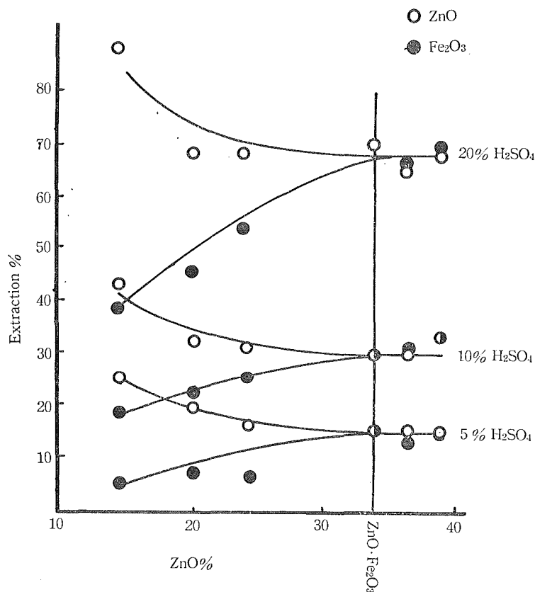
Fig. 4 Relation between extraction and composition.
