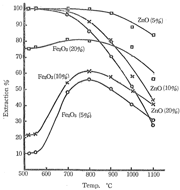
Fig. 3 Acid extraction curves for calcined samples.
