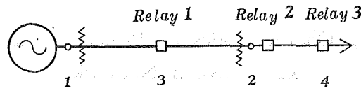
Fig. 7. Impedance Relay.
