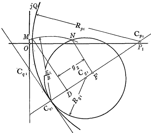
Fig. 5. Conductance circle and graphical method to ob- tain g_2 .
