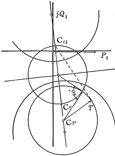
Fig. 6. Apparent admittance or impedance circles.
