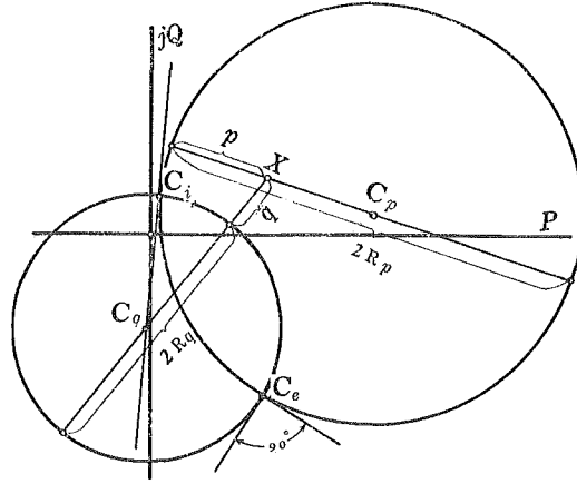
Fig. 3. Circle co-ordinate C_p and C_q circles intersecting at rectangle.
