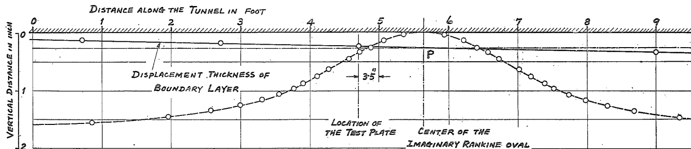
FIG. 14 VARIATION OF THE DISPLACEMENT THICKNESS OF BOUNDARY LAYER ALONG THE WIND-TUNNEL AND THE ESTIMATED FORM OF THE CEILING AND THE BOTTOM
