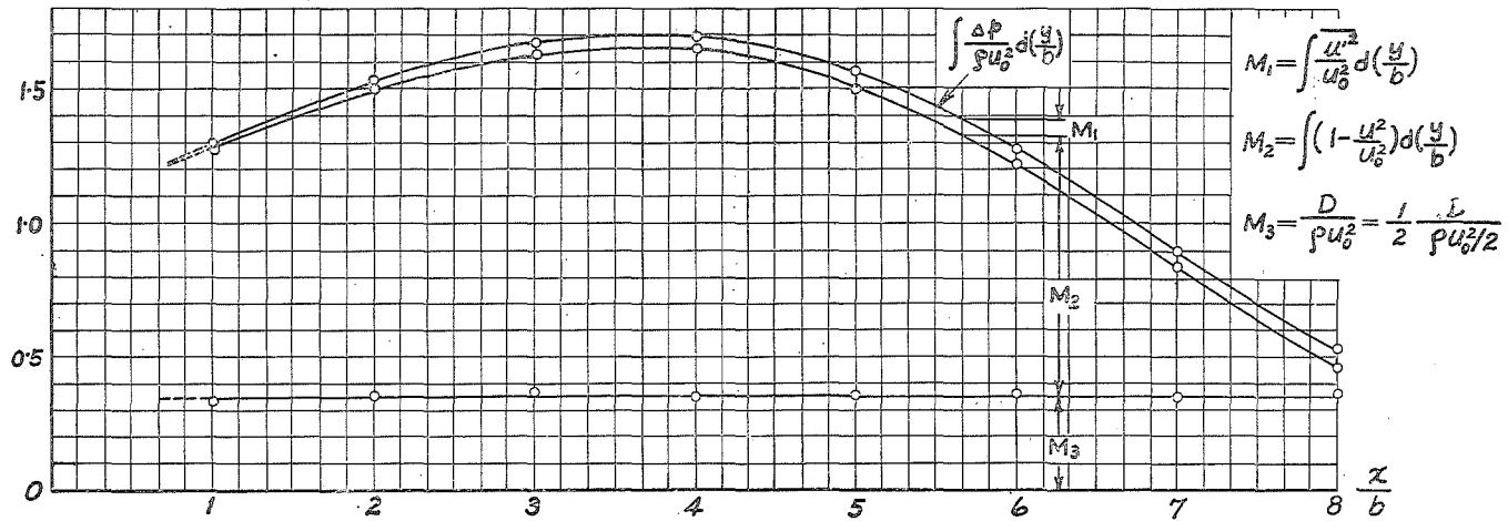
Fig. 40 Distribution of shear force behind a normal plate in contact with a boundary
