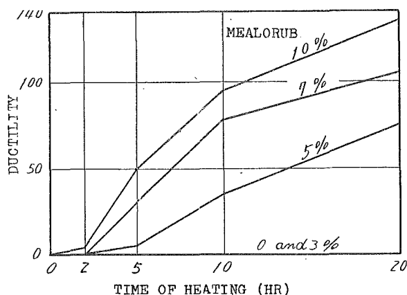
Fig. 4. Relation between ductility at 0°C and heating time of the blend with natural rubber powder "Mealorub".
