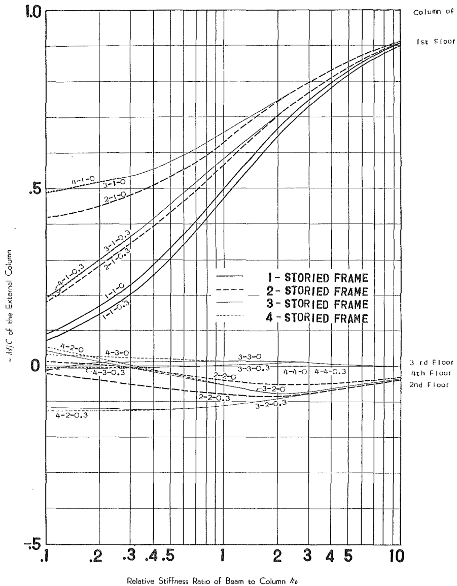
Fig. 3 (a). Thermal bending moments at the top of the most external column of the frame.
