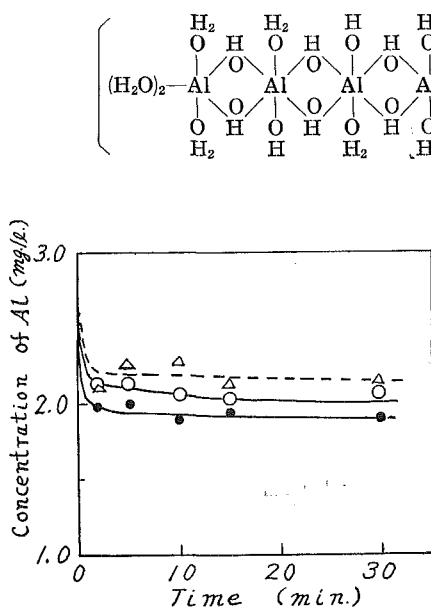
Fig. 6. Changes in the concentration of aluminum capable of passing through filter paper.
