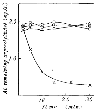
Fig. 13. Effect of monomeric silica. pH, 6.2 \pm 0.2 ; initial concentration of Al, 2.6 mg./l.; concentration of added in mg./l., \square 0, \Delta 10, \circ 20, and \times 50.
