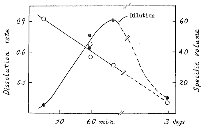
Fig. 10. Changes in dissolution rate and specific hydrodynamic volume during the aging of Baylis sol. ○ dissolution rate; ● specific volume.
