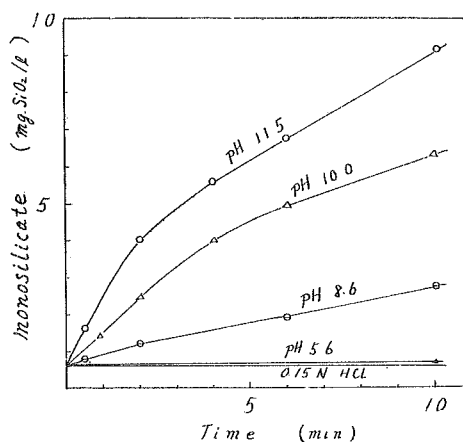
Fig. 3. Dissolution of colloidal silica particles at various pH values. Total SiO 2 , 18.5 mg./l.; pH adjusted with Na 2 CO 3 and NaHCO 3 .
