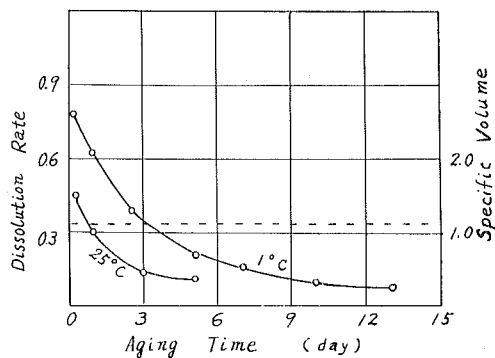
Fig. 9. Changes in dissolution rate and specific hydrodynamic volume during the aging of ion-exchanged sol. —○—○— dissolution rate; ..... specific volume.
