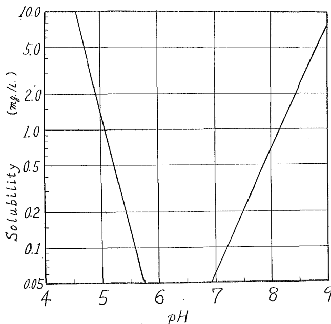
Fig. 5. Solubility of Al ion at 25°C.
