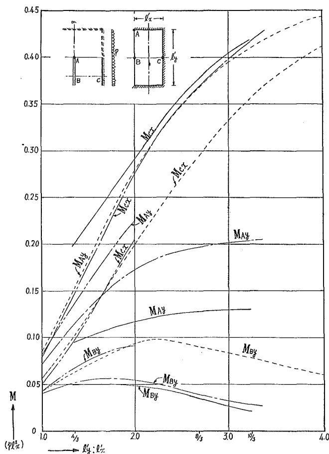
Fig. 21. k^4=3 n=4/3 \left\{ \begin{array}{l} \text{Dobashi} \\ \text{Yokoo} \end{array} \right\} Four-edge fixed anisotropic in flight Anisotrop. k^4=1 n=1 \left\{ \begin{array}{l} \text{Yokota} \\ \text{Higashi} \end{array} \right\} Three-edge fixed one-edge free } Plain isotrop. All under uniform load.
