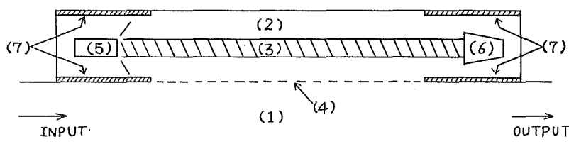
Fig. 1. Sketch of traveling-wave tube coupled with directional coupler:
