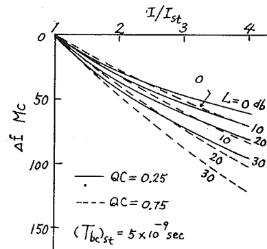
Fig. 4. I/I_{st} vs \Delta f with L as parameter
