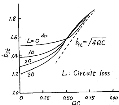
Fig. 1. Theoretical curves of b_{st} vs QC at start oscillation
