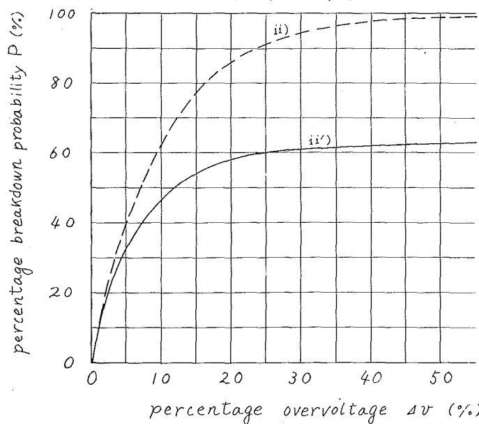
Fig. 5 b. Is the reproduction of ii) and ii') in Fig. 5 a with different scale of abscissa, ii') never reaches 100%.
