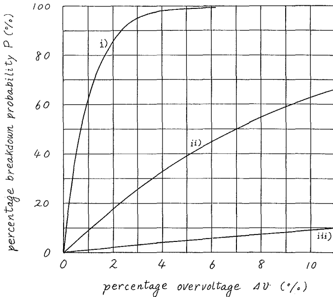
Fig. 1. Showing P to \Delta v relationship of parallel plane gap with rectangular pulse applied i) nsLT=10^2 , ii) 10^1 , iii) 10^0
