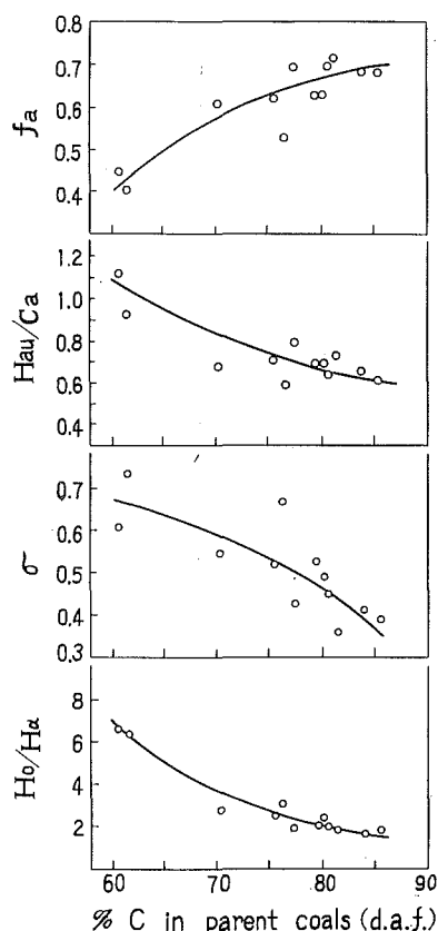
Fig. 4. A plot of f_a , H_{au}/C_a , \sigma and H_o/H_a for the pyridine extracts of coals against the carbon content of the parent coals
