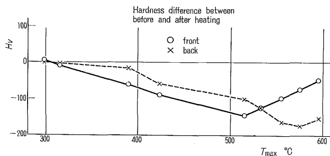
Fig. 27. Hardness difference between before and after heating
