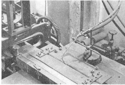
Fig. 1. Roll Stretcher and Heat Tensioning Apparatus
