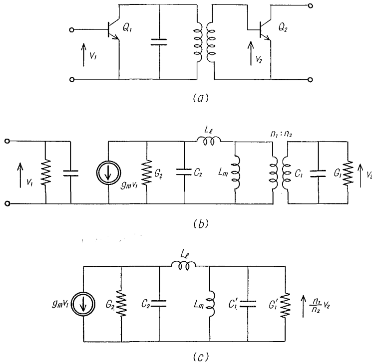
Fig. 2. Transformer-coupled Tuned Amplifier
