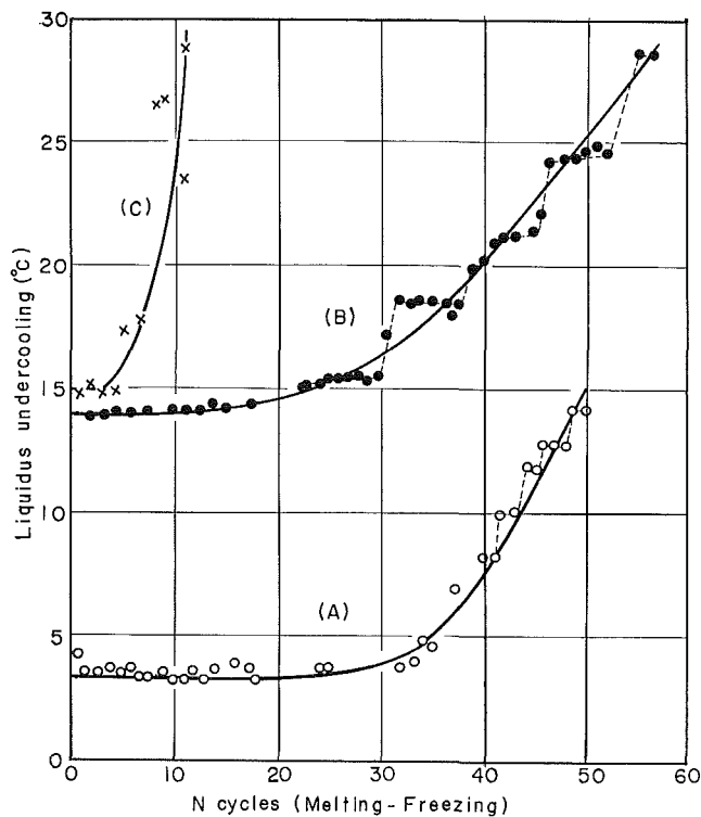
Fig. 5. Relation between degree of liquidus undercooling and cycle number ( N ) of melting-freezing in Al-4 wt. % Cu alloy.
