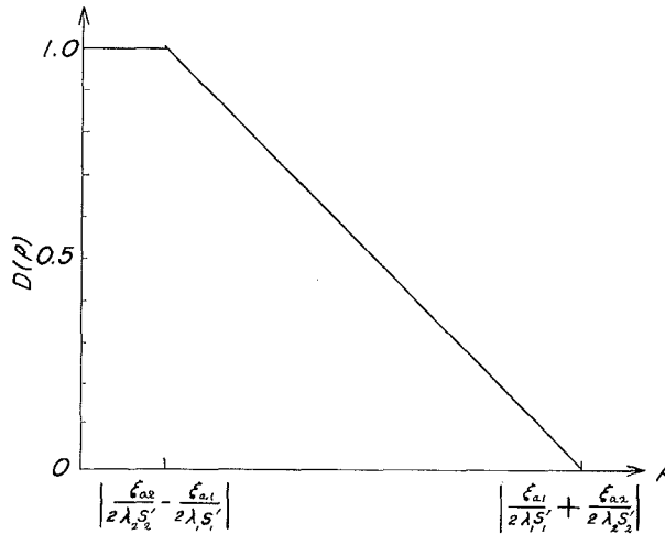
Fig. 10. Plot of convolution integral for Eq. (77).
