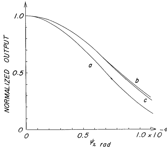
Fig. 7. The theoretical normalized output [D(\psi_2)/D(0)]^2 vs \psi_2 in the case where \theta_1 = \varphi_1 = \pi/2 and \delta_2 = 0 at 6328 \text{ \AA} ; (a) the rectangular detector of sides a=b=0.4 \text{ cm} , (b) the circular detector of radius \rho_0=0.2 \text{ cm} , and (c) the rectangular detector of the same area with (b).
