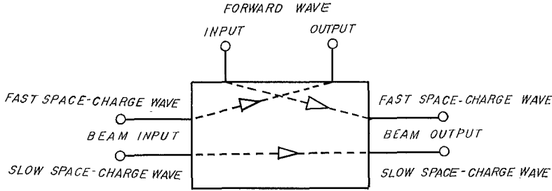
Fig. 1. Block diagram of a Kompfner null coupler.
