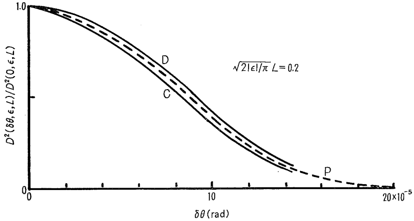
Fig. 4. The effect of beam tilt on signal power output; (C) converging wavefronts, (D) diverging wavefronts, and (P) plane waves, in the case where \sqrt{2|\epsilon|/\pi} L = 0.2, \theta_1 = 0, \theta_2 = \delta\theta and L = 3 \text{ mm} at 6000 \text{ \AA} and \epsilon = 0 for plane waves.
