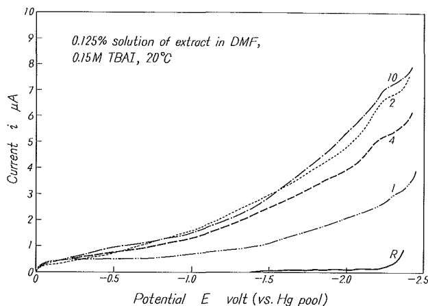
Fig. 2. Polarograms for the extract solutions of identical concentration.
