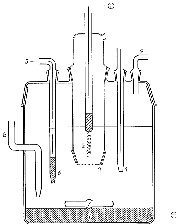
Fig. 1. Electrolytic cell
