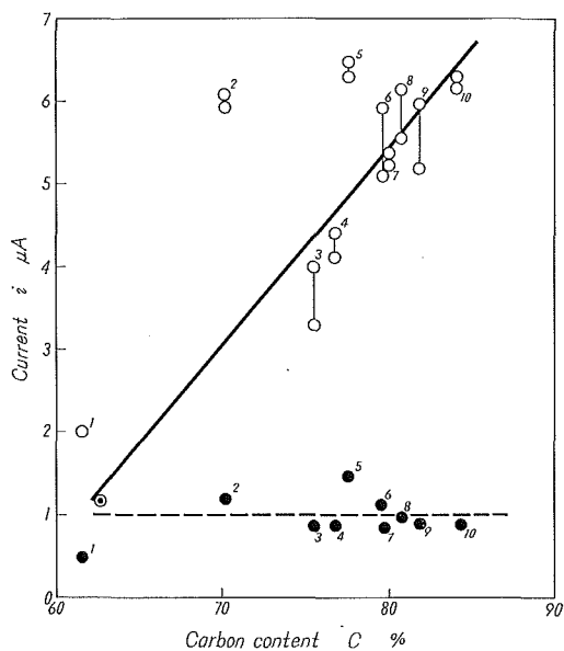
Fig. 5. Change of polarographic current with the carbon content of original coals. concentration of extract: 0.125 w/v %.
