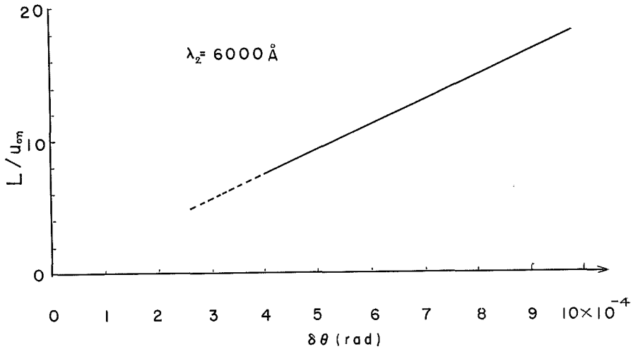
Fig. 5. The angular selectivity of \delta\theta for D_g = 1/\sqrt{2} in the case in which \theta_1 = 0 , \theta_2 = \delta\theta , and u_{01} = u_{02} = u_{0n} at 6000 Å.
