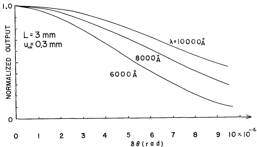
Fig. 6. The theoretical normalized output with optical wavelengths as the parameter. It was assumed that u_{0n} = 0.3 mm, L = 3 mm, \theta_1 = 0 and \theta_2 = \delta\theta .
