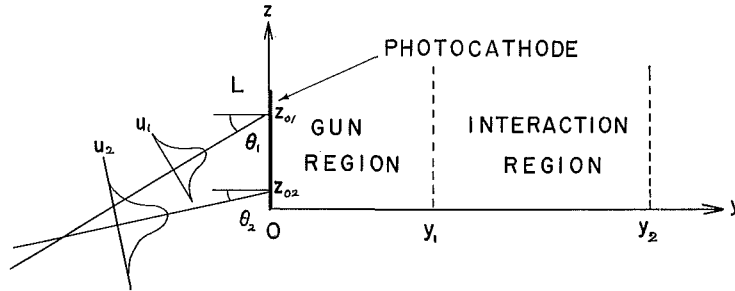
Fig. 2. Representation of detection process with Gaussian plane waves.
