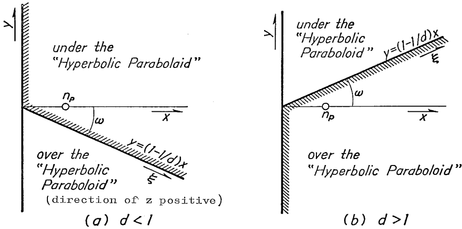
Fig. 1. Boundary Plane and Axis \xi
