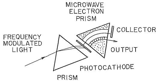
Fig. 1. Schematic of microwave electron prism.
