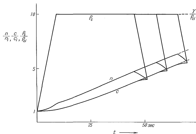
Fig. 5. Optimum Controls and corresponding trajectories of the several objective powers.
