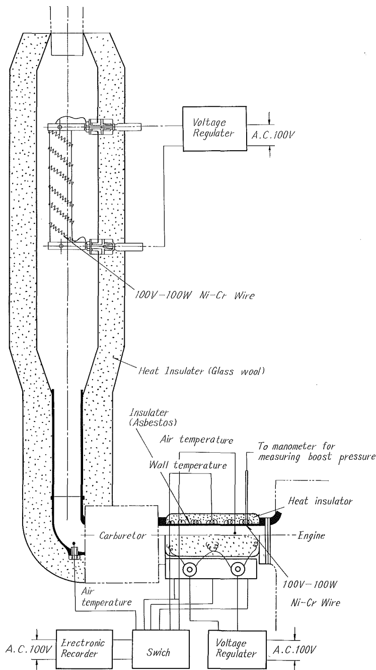
Fig. 1. The heating apparatus of intake air and mixture
