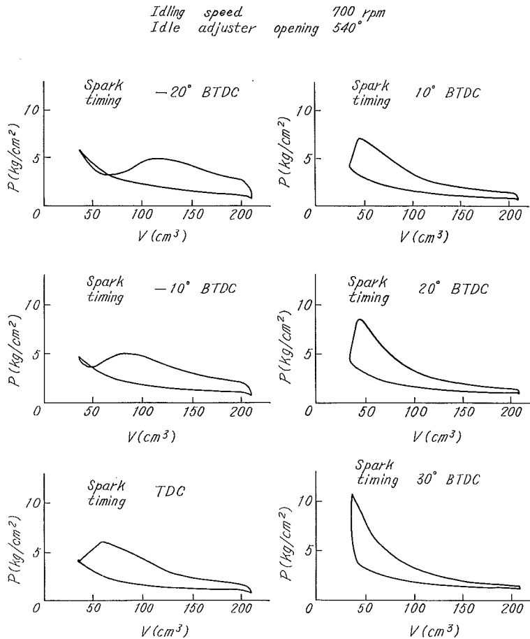
Fig. 6. Indicator diagram under the varied spark timing (Idling speed 700 rpm, Idle adjuster opening 540°)
