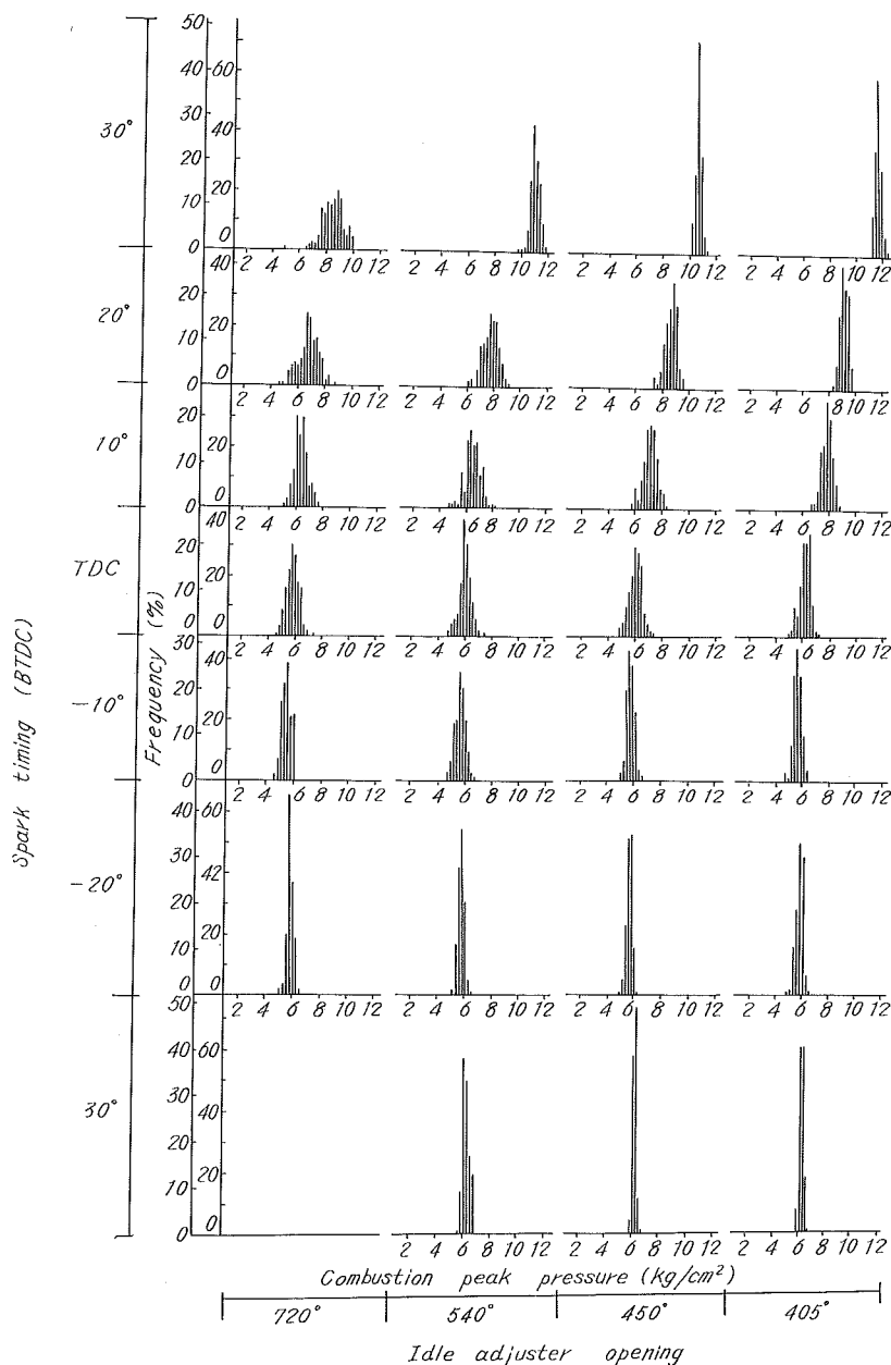
Fig. 13. The frequency distribution of combustion peak pressure
