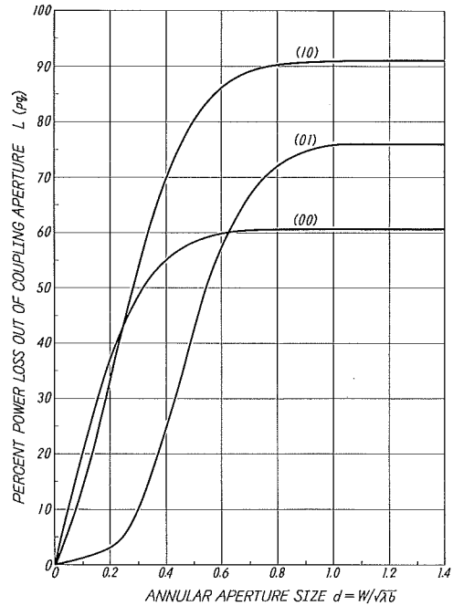
Fig. 2. Percent power loss versus annular aperture size for the TEM_{00} , TEM_{10} , and TEM_{01} modes with r_0^2 = R_0^2/2 = 1/4\pi .
