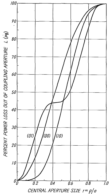
Fig. 10. Percent power loss as a function of radius of the central aperture for the TEM_{00} , TEM_{10} , and TEM_{01} modes.
