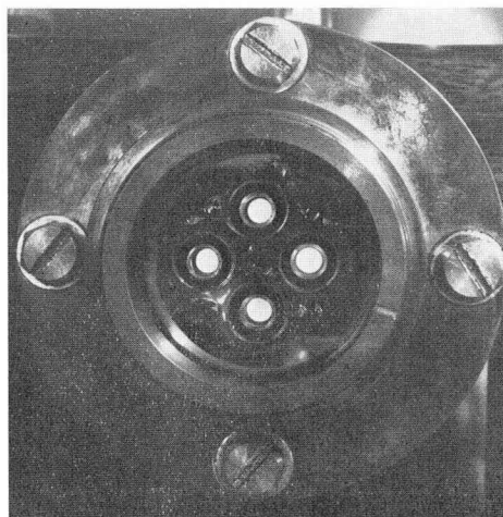
Fig. 11. The plane mirror with four coupling holes mounted on the laser tube.
