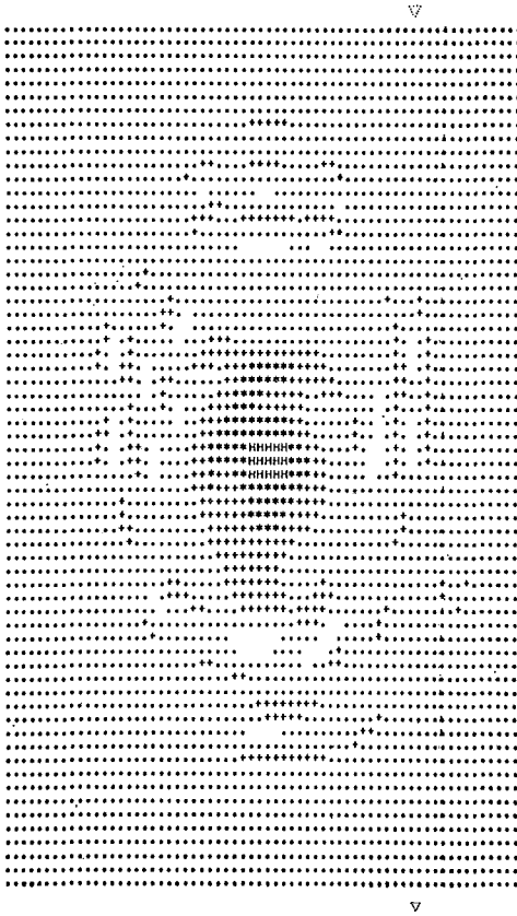
Fig. 17. Intensity distribution of the array function. The intensity a_R (normalized) is digitized into five levels as expressed by the letter and symbols, H ( a_R \geq 1.0 ), * ( 1.0 > a_R \geq 0.75 ), + ( 0.75 > a_R \geq 0.5 ), \cdot ( 0.5 > a_R \geq 0.25 ), and blank ( 0.25 > a_R ).
