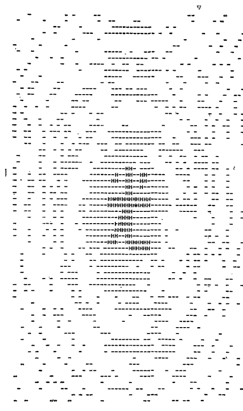
Fig. 18. Image numerically synthesized in the Fresnel transform plane by the array described by the array function of Fig. 17.
