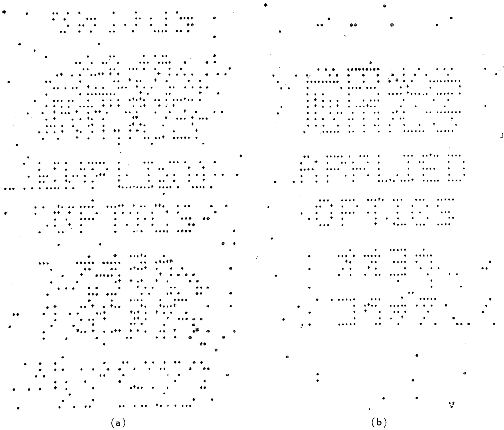
Fig. 15. Numerically synthesized images, where a is due to one array function and b is the intensity average of six images which are synthesized by the temporal array describing six different array functions obtained by the procedure of Fig. 14.
