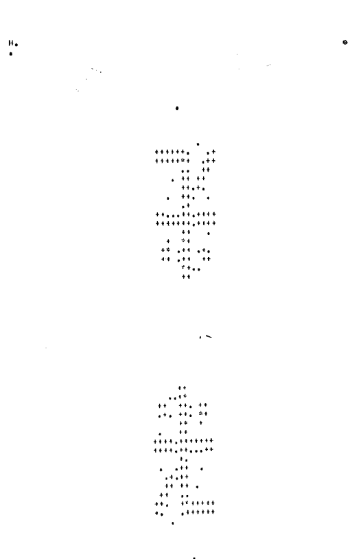
Fig. 6. Images numerically synthesized by the digital amplitude arrays of Fig. 5. The strong field distribution (displayed by the letter H ) appears at the origin of the image plane (at the top left corner).
