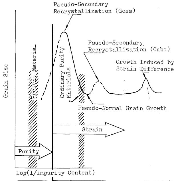
Fig. 1. Schematic representation of modes of grain growth. Grain size against impurity content (C) with strain complementary to it.
