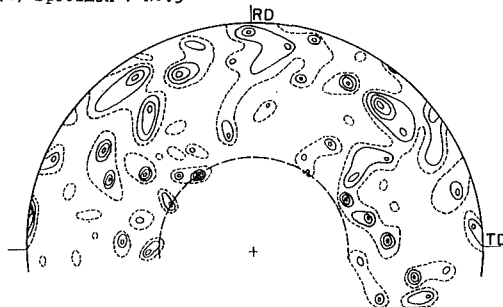
Fig. 4. (110)-pole figures of cold rolled 3.17% Al-Fe alloy sheets annealed at 1200°C for 1 hr in hydrogen atmosphere.
