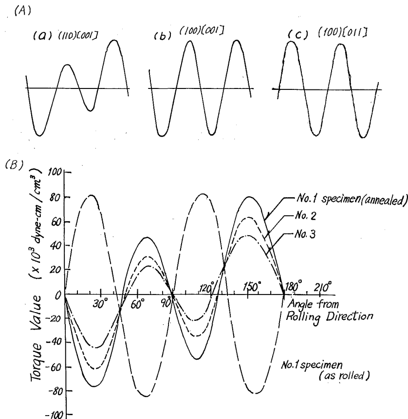
Fig. 5. Torque curves of a few typical single crystals (A) and of cold rolled 3.17% Al-Fe alloy sheets of as rolled and annealed at 700°C for 1 hr in hydrogen atmosphere (B).
