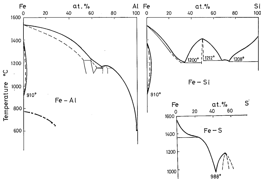
Fig. 8. Phase diagrams of alloy system of Fe-Al, Fe-Si and Fe-S (20) .
