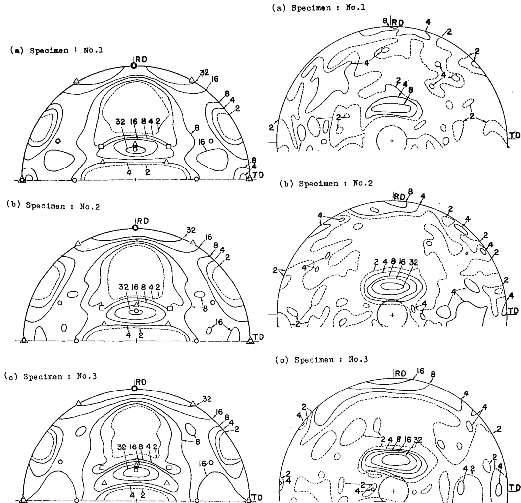
Fig. 1. (110)-pole figures of cold rolled 3.17% Al-Fe alloy sheets by 70% to 3.5 mm in thickness. Symbols \triangle , \circ and \square indicate (111) [11 \bar{2} ], (112) [1 \bar{1} 2] and (100) [011] poles respectively.
