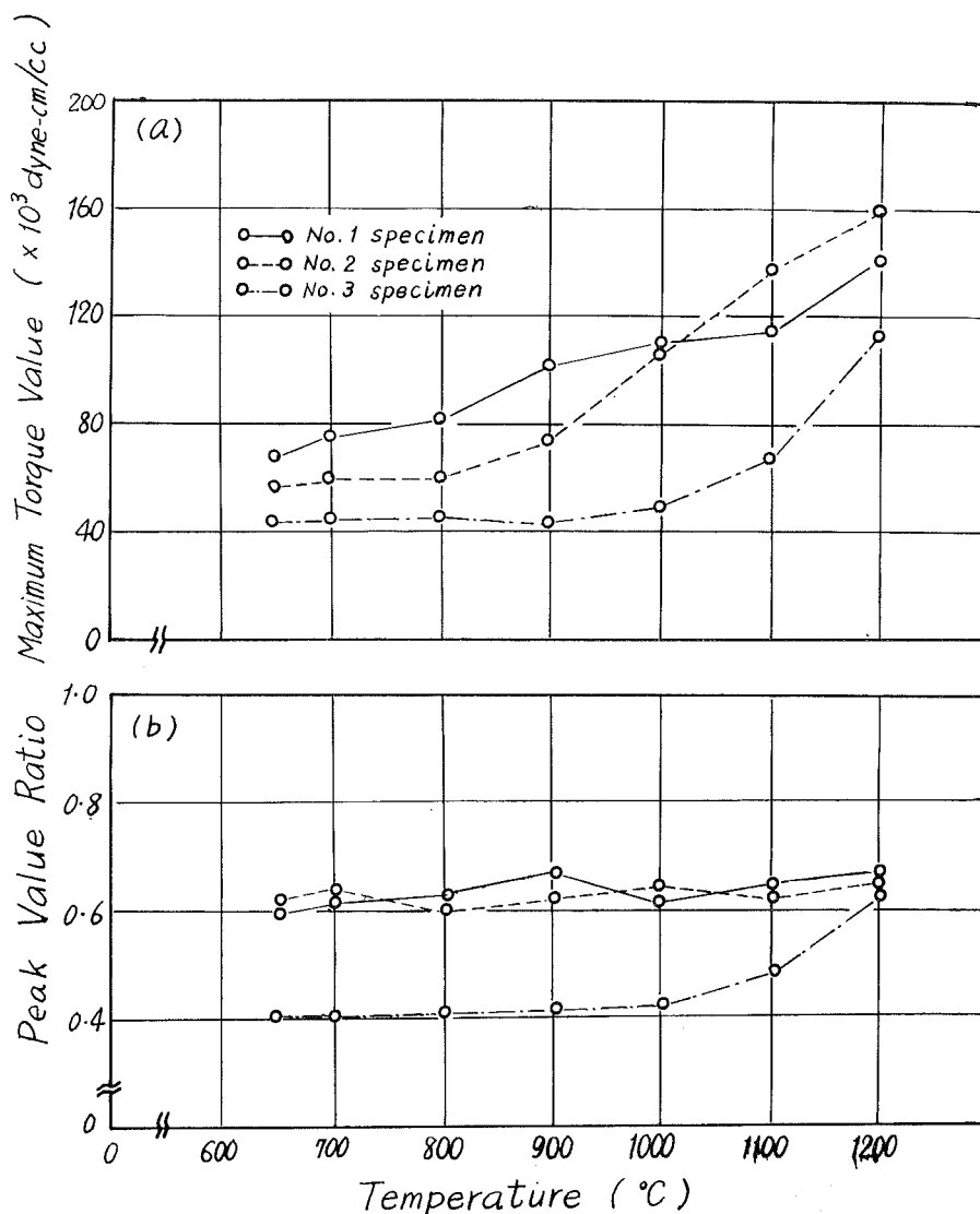
Fig. 6. Maximum torque values (a) and peak value ratios (b) of cold rolled 3.17% Al-Fe alloy sheets annealed at various temperatures for 1 hr in hydrogen atmosphere.
