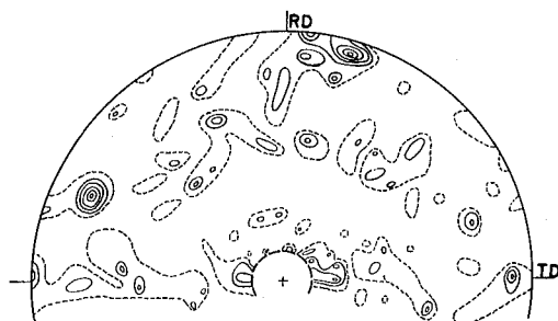
Fig. 3. (100)-pole figures of cold rolled 3.17% Al-Fe alloy sheets annealed at 1200°C for 1 hr in hydrogen atmosphere.
