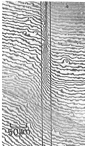
Fig.1 (a) Interference micrograph showing gradient of surface bending around a twin. The surface bending was measured on the two lines parallel to the twin. (b) Schematic diagram showing surface bendings around a twin.
