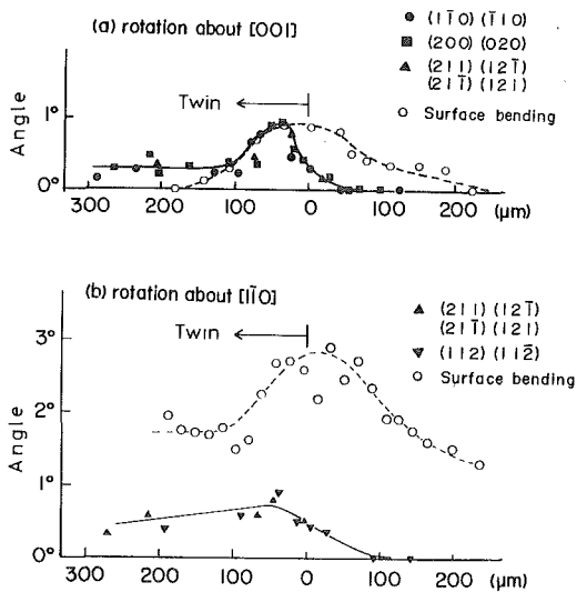
Fig.3 Surface bending and lattice rotation around the twin in Fig.2(a). The abscissa is the distance from the tip of twin measured parallel to the trace of twin, [\bar{1}10]
