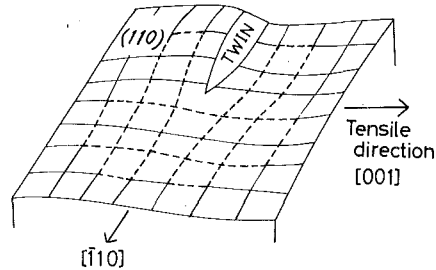
Fig.1 (a) Interference micrograph showing gradient of surface bending around a twin. The surface bending was measured on the two lines parallel to the twin. (b) Schematic diagram showing surface bendings around a twin.
