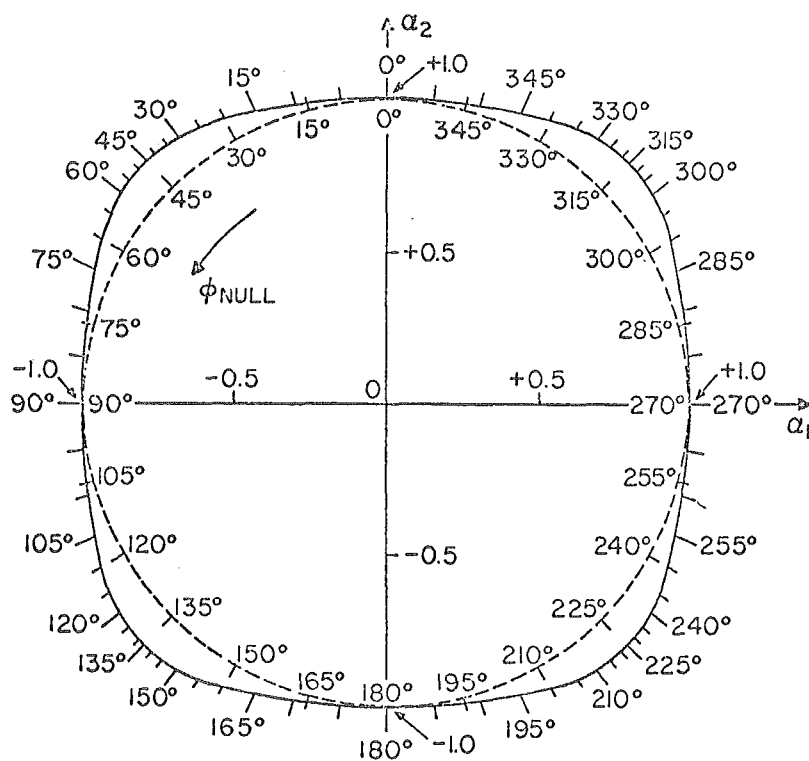
Fig. 4. Loci for \phi_{\text{null}} in \alpha_1\alpha_2 -plane — Monopole and crossed \lambda/2 slots - - - Monopole and crossed magnetic dipoles.
