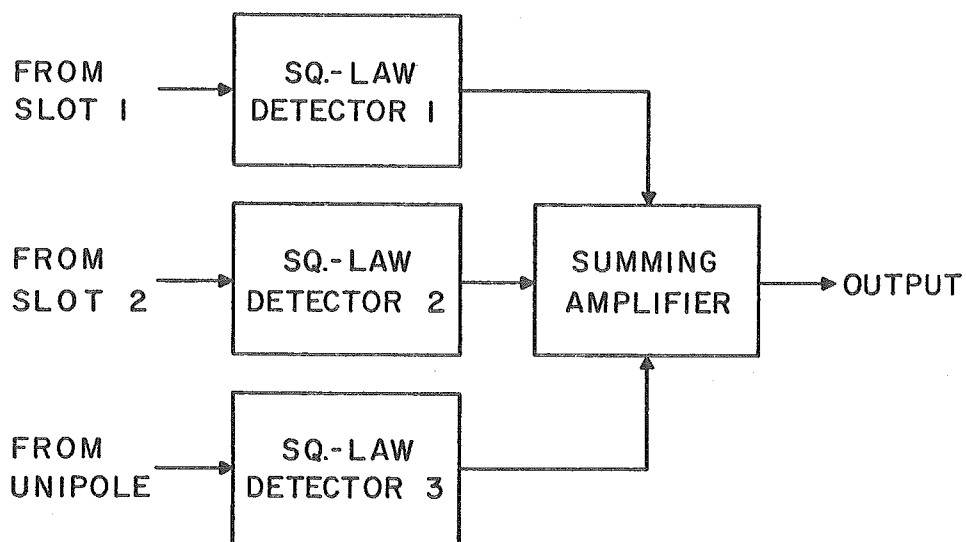
Figure 2. Processing circuit for energy-density antenna.
