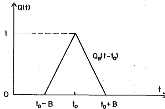
Fig. 1 Triangular pulse in output.
