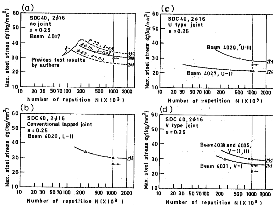
Fig.11 Fatigue test results, \sigma_s - N diagrams
