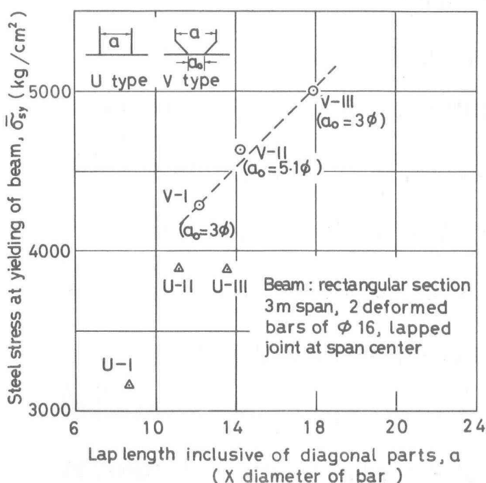
Fig.8 Relationship between beam strength and lap length of V type joint
