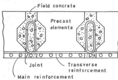
Fig.3 U-shaped lapped joint
