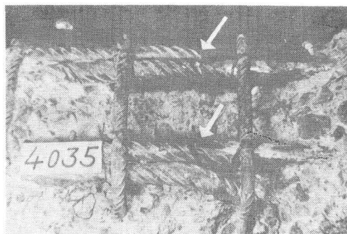
Fig.10 Fatigue fracture of deformed bars
