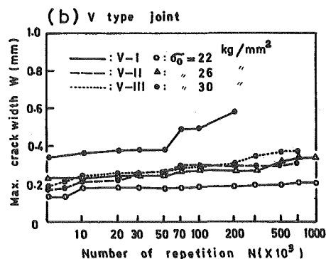
Fig.13 Maximum crack width in beam under repeated load
