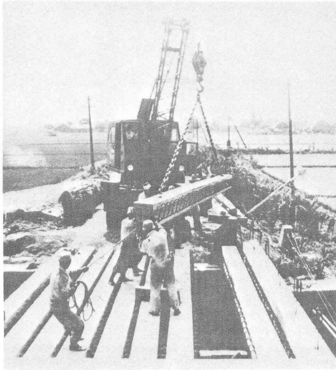
Fig.2 Precast concrete slab bridge under construction
