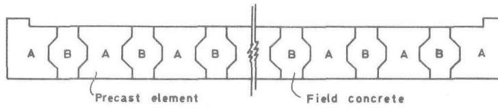
Fig.1 Section of precast concrete slab bridge
