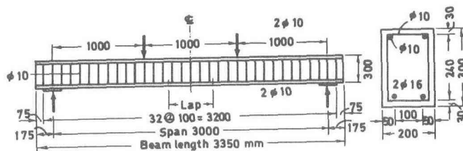
Fig.6 Test beam
