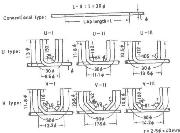
Fig.7 Details of bar joints
