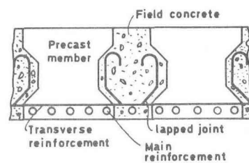
Fig.4 V type lapped joint
