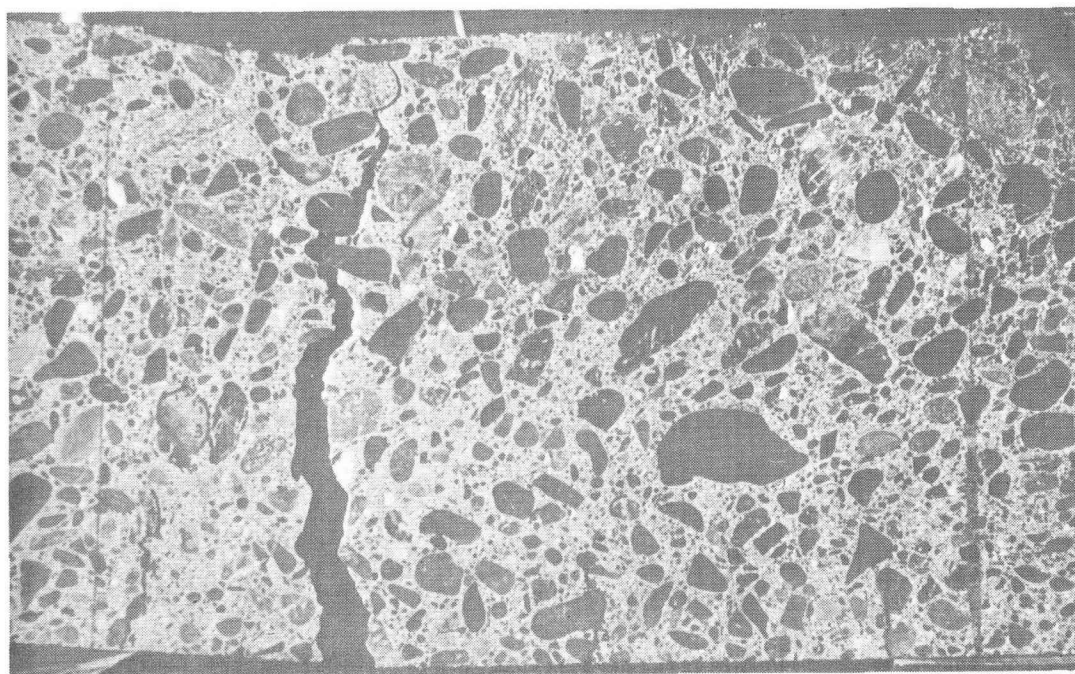
Fig. 5 Crack of concrete beam after failure at load, 2.415 tons
