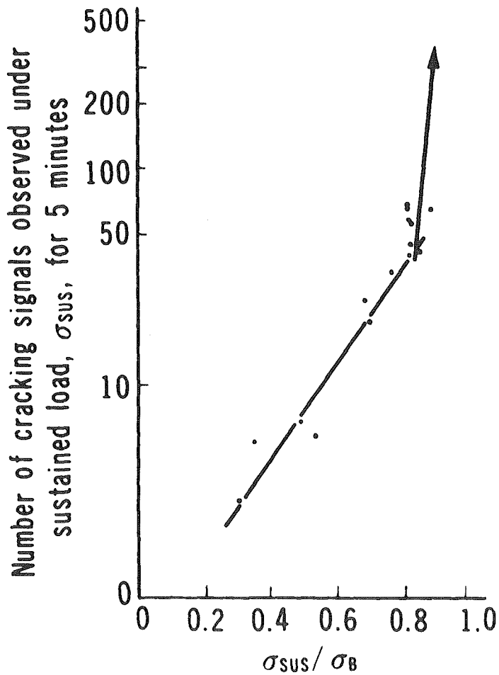
Fig. 7 Number of cracking signals vs. sustained load
