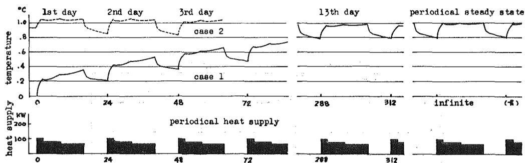
Fig. 6 Intermittent heat supply and calculated room air temperature
