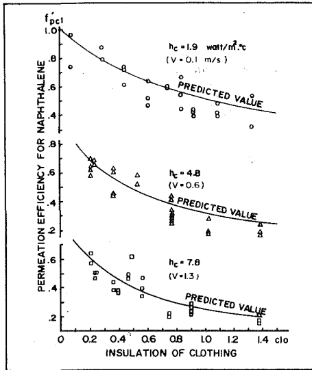
Fig. 3 Comparison between experimentally derived permeation efficiency factors for naphthalene transfer and theoretically predicted values. Air movement was adjusted so that the convective heat transfer coefficient at the testing surface was h_c = 1.9 , 4.8 and 7.8 \text{ W } (m^2 \cdot ^\circ C) , which values are equivalent to 0.1 , 0.6 and 1.3 \text{ m/s} , respectively.
