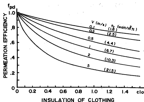
Fig. 1 The relation between the theoretically derived permeation efficiency factor for water vapor transfer, f_{pcl} , clo value and the air movement. The factor, f_{pcl} , takes the ultimate value of 1.0 in the unclothed condition at any air movement.
