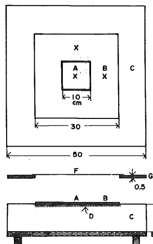
Fig. 2 Design of experimental apparatus. This apparatus, used for the measurement of thermal insulation and sublimation, consists of a pair of two identical plates – heated copper plate and naphthalene plate.
