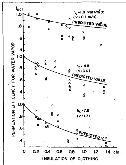
Fig. 4 Comparison between permeation efficiency factors for water vapor transfer and theoretically predicted values. Permeation efficiency factors for water vapor were derived from naphthalene data, shown in Fig. 3, using the analogy of mass transfer processes.
