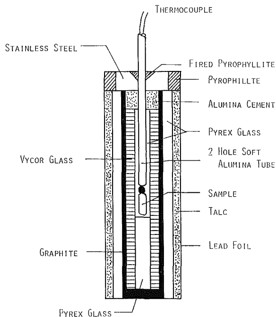
Fig. 1. Schematic diagram of glass cell assembly.
