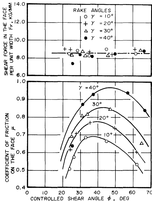
Fig. 4. Shear force in the face and apparent coefficient of friction in controlled shear angle cutting tests.
