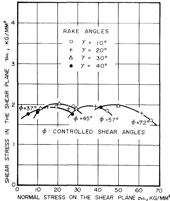
Fig. 5. Shear stress in the shear plane \tau_{shi} versus normal stress on the shear plane \sigma_{shi} in controlled shear angle cutting tests.
