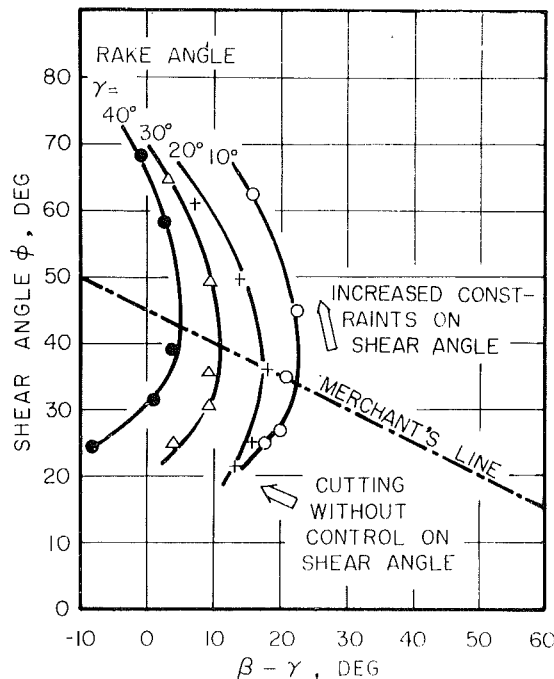
Fig. 7. Correlation between shear angle \phi and (\beta - \gamma) in controlled shear angle cutting tests.
