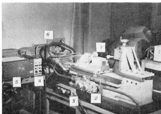
Fig. 1. Arrangement for artificially controlled shear angle cutting test.
