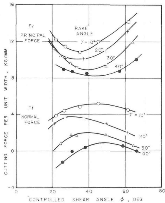
Fig. 3. Measured cutting force in controlled shear angle cutting tests.
