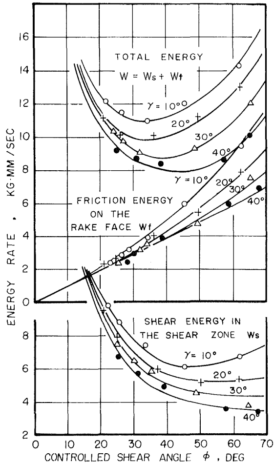
Fig. 6. Shear deformation energy rate in the shear zone W_s , friction energy rate on the rake face W_f , and total energy rate W = W_s + W_f in controlled shear angle cutting tests.
