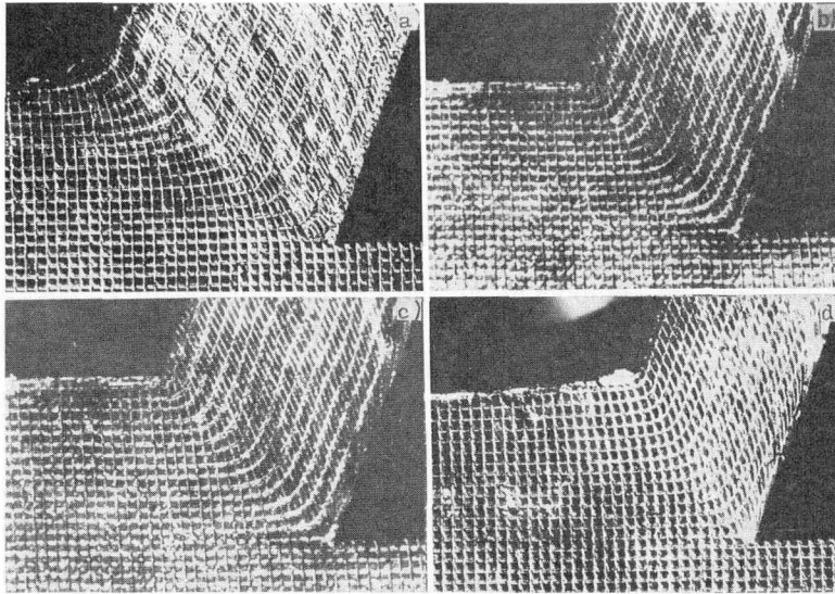
Fig. 2. Photographs of partially formed chips in free and controlled shear angle tests.
