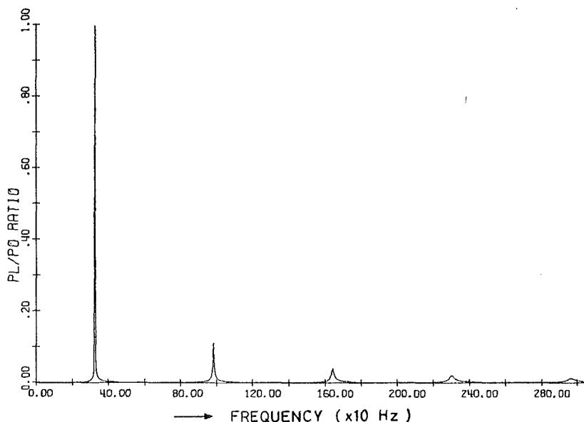
Fig. 3. Frequency response p_i/p_o(\omega) of a closed tube, calculated from the values: radius a=0.80 cm, length l=25.0 cm, at temperature 10^\circ\text{C} .
