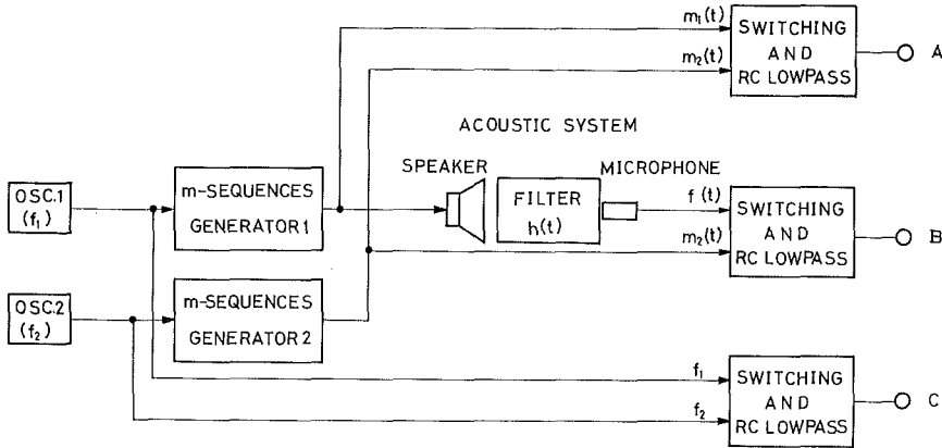
Fig. 2. The block diagram of the stroboscopic correlation method using the signal of m -sequences.
