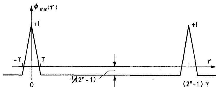
Fig. 1. Autocorrelation function of an m -sequence signal.
