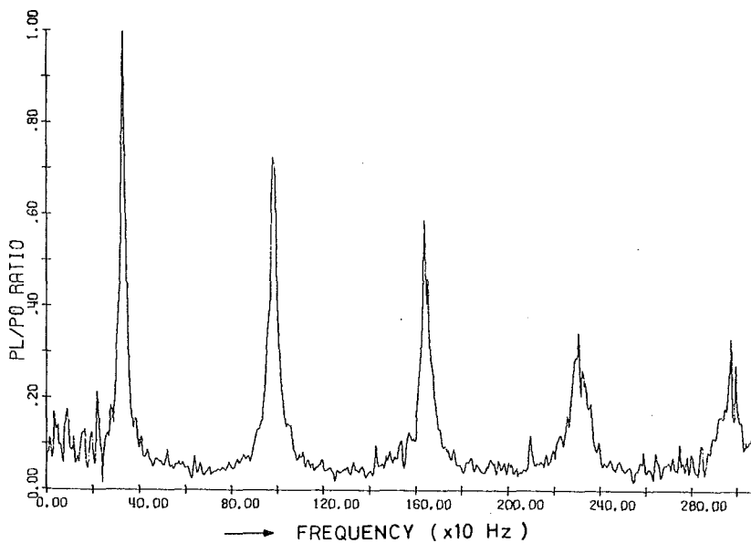
Fig. 5. The measured frequency response p_l/p_o(\omega) of a closed tube: radius a=0.80 cm, length l=25.0 cm, at room temperature 10^\circ\text{C} . The signal of an m -sequence used: period N=2^{11}-1=2047 shift pulse frequency 10 kHz.
