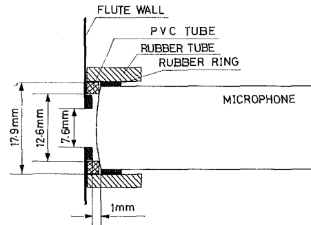
Fig. 8. A fitting of a condenser microphone to a finger hole of the flute.
