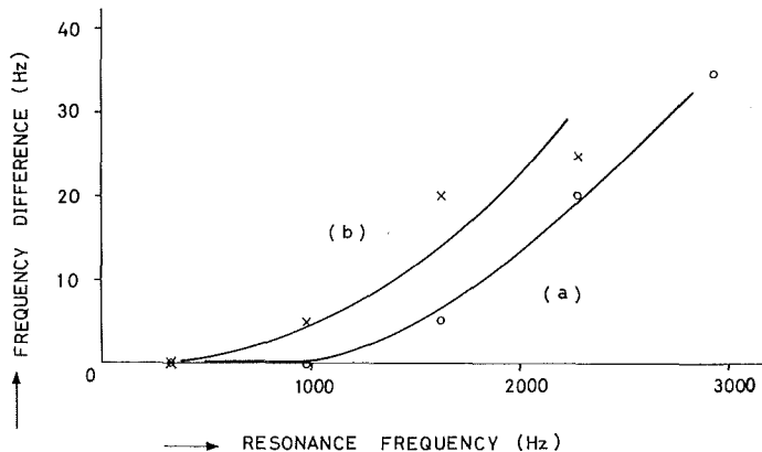
Fig. 6. Higher harmonics of a closed tube differ from the integral multiples of the fundamental resonant frequency. Curve (a): with baffle. Curve (b): without baffle.
