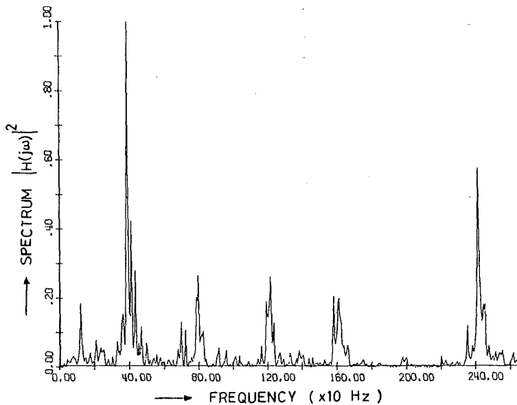
Fig. 12. Frequency response of the flute. Some finger holes were closed according to G-fingering (392 Hz). Sound source: at the third finger hole. Microphone: at the mouth hole.
