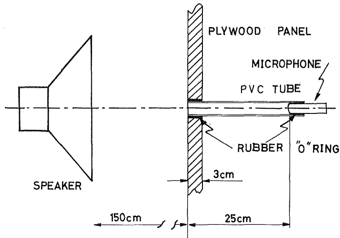
Fig. 4. The setup used to determine the resonances of a closed tube with a large baffle plate.
