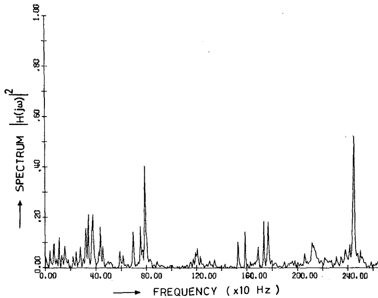
Fig. 11. Resonances were not observed in the flute tone range, when the microphone was placed at a few centimeters from the tail end, outside of the flute. Sound source: at the B-hole. Fingering: A (440 and 880 Hz by overblowing).
