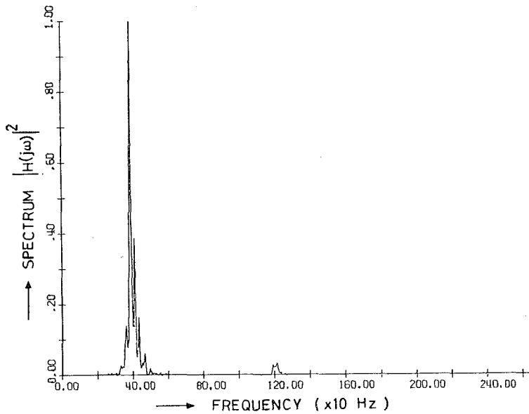
Fig. 9. Resonance of the flute was seen at 392 Hz when some finger holes were closed according to G-fingering (392 Hz). Sound source was placed at the third finger hole, microphone at the B-hole.
