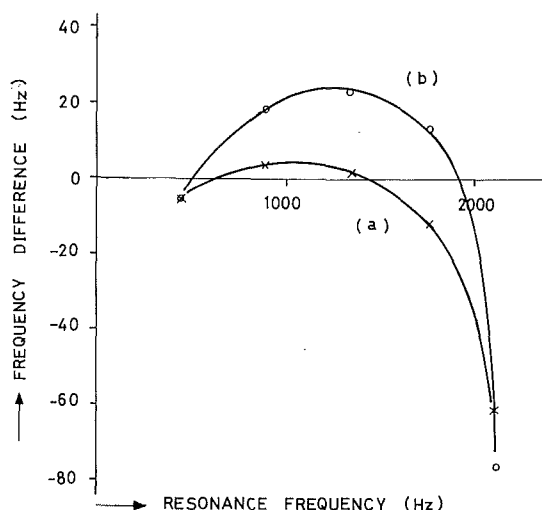
Fig. 13. Frequencies of the higher harmonics differed from the integral multiples of the fundamental frequency of the flute. Curve (a): frequency difference when the mouth hole was partially covered. Curve (b): frequency difference with this coverage removed. Sound source was placed at the mouth hole and the microphone was in place of the stopper. Some finger holes were closed according to A-fingering (440 and 880 Hz by overblowing).
