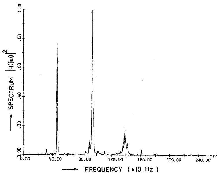
Fig. 10. Resonances of the flute were seen at 459 Hz and at 942 Hz. Some finger holes were closed according to A-fingering (440 and 880 Hz by overblowing). Sound source was placed at the B-hole, microphone was in place of the stopper.
