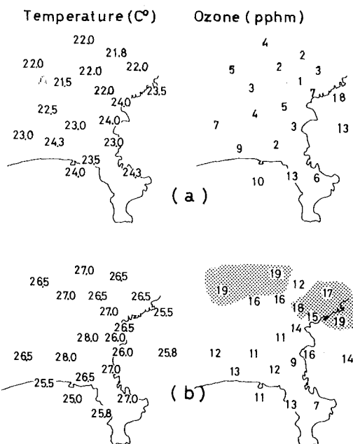
Fig. 8. Horizontal distribution of ozone concentration and temperature at the altitude of 300 m on July 19, 1973. Fig. (a) and (b) are observed at 0935-1106 and 1327-JST respectively.
