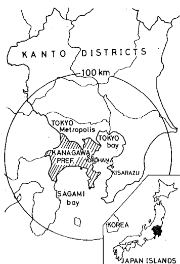
Fig. 1. Map of Kanagawa prefecture and its vicinity.
