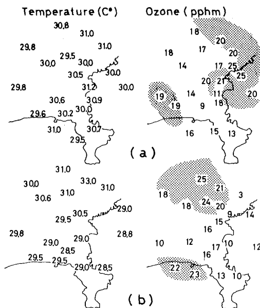
Fig. 7. Horizontal distribution of ozone concentration and temperature at the altitude of 300 m on July 18, 1973. Fig. (a) and (b) are observed at 0940-1106 and 1324-1439 JST respectively.
