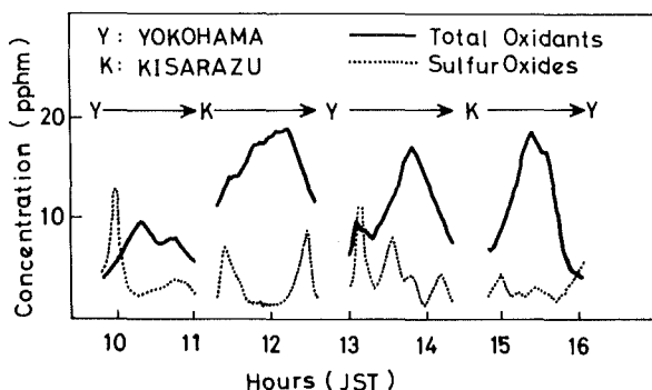
Fig. 9. Distributions of oxidants and sulfur oxides observed on a ferry boat between Yokohama and Kisarazu on August 9, 1971.
