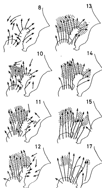
Fig. 3. Air flow pattern and distribution of oxidants near the ground on July 17, 1973. Hatched area indicates the area of more than 10 pphm of oxidants. Numerals in the figure are the time of observation in JST.
