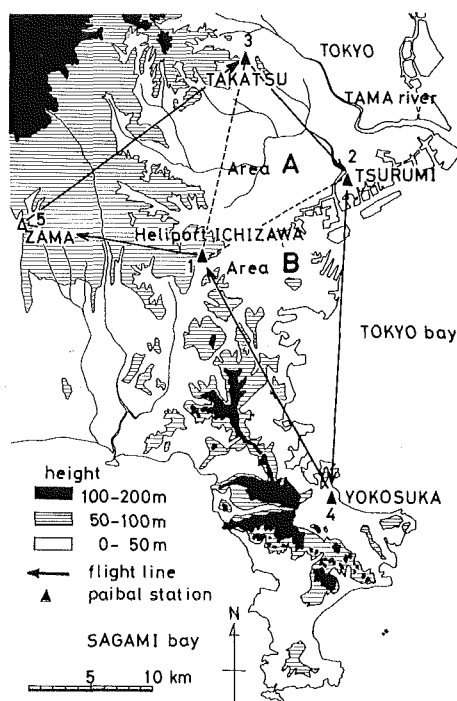
Fig. 2. Topography of observational area.
