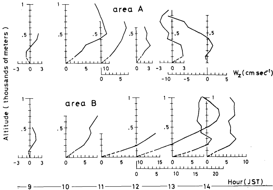
Fig. 5. Distribution of vertical velocity W_z on July 17, 1973.
