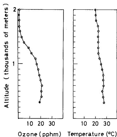
Fig. 6. Ozone distribution observed up to 2000 m at Zama between 1349 and 1358 JST on August 28, 1973.
