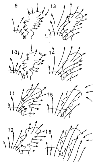
Fig. 10. Air flow pattern near the ground on August 9, 1971. Numerals in the figure are the time of observations in JST.
