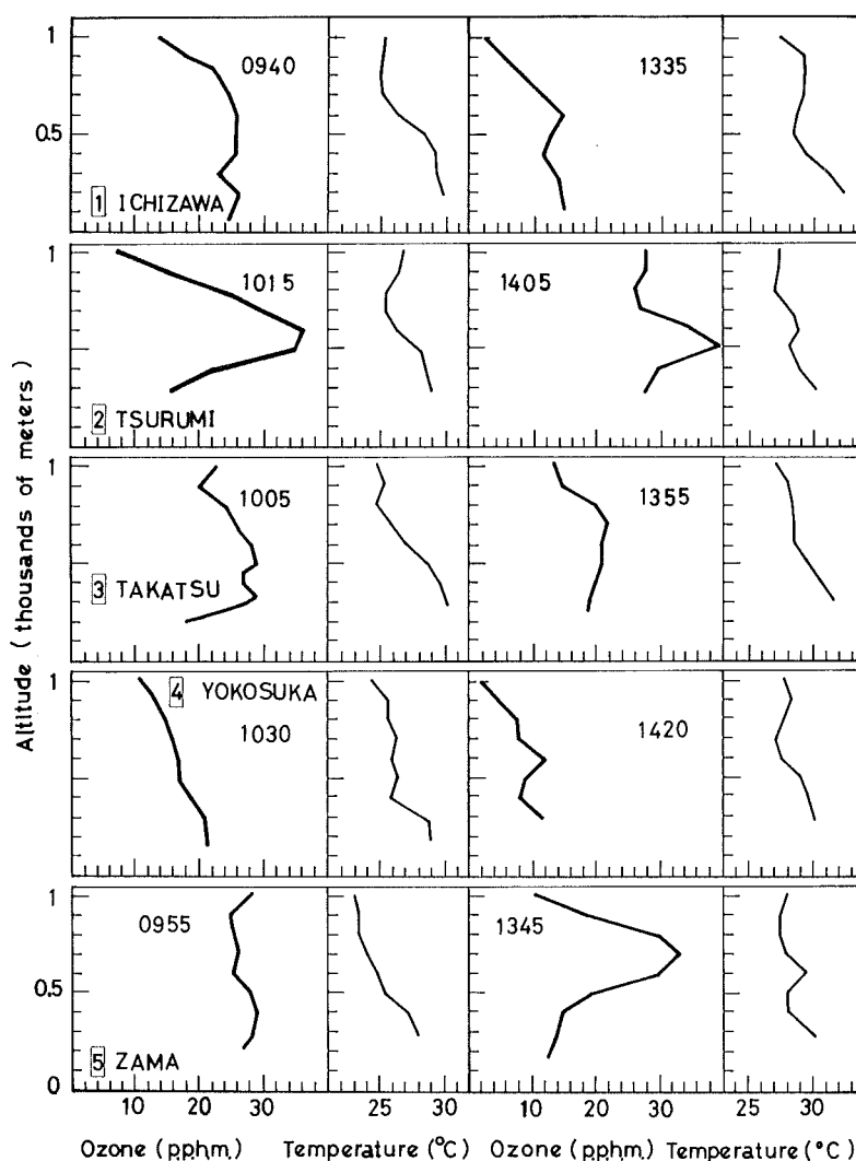
Fig. 4. Vertical distributions of ozone and air temperature on July 17, 1973. Numerals in the figure are the time of observations in JST.
