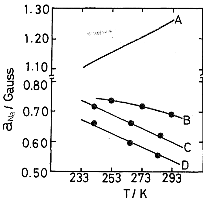
Fig. 7. Temperature dependence of hyperfine splitting due to counteranion in ESR spectra of pyrazine anion (A) ion-pairing with \text{Li}^+ in tetrahydrofuran 14) , (B) with \text{Na}^+ in tetrahydrofuran containing hexamethylphosphorotriamide, (C) with \text{Na}^+ in tetrahydrofuran and D with \text{Na}^+ in dimethoxyethane.
