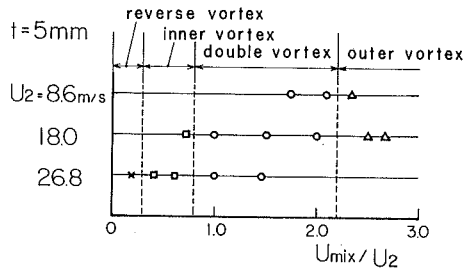
Fig. 13. Change of flow pattern against U_{mix}/U_2 .
