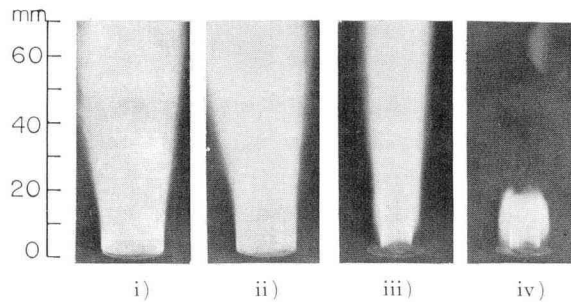
Fig. 4. Photographs of flame geometries
