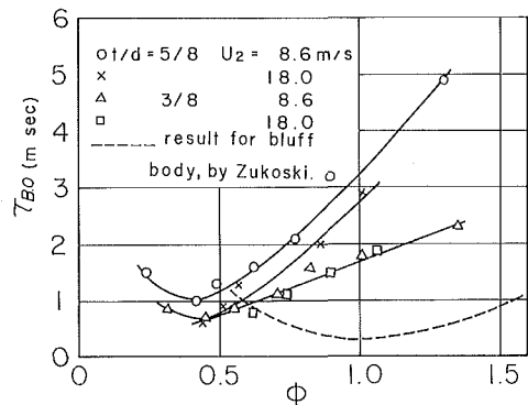
Fig. 10. Critical ignition delay time.
