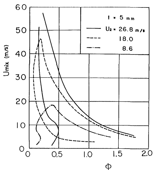
Fig. 8. Effects of U_2 on stability limits.
