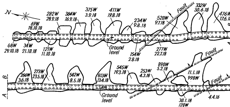
Fig. 1.5) Outbursts of \text{CO}_2 in Level Gallery of Ferdinand Seam, Ruben Colliery (by Wilson)
