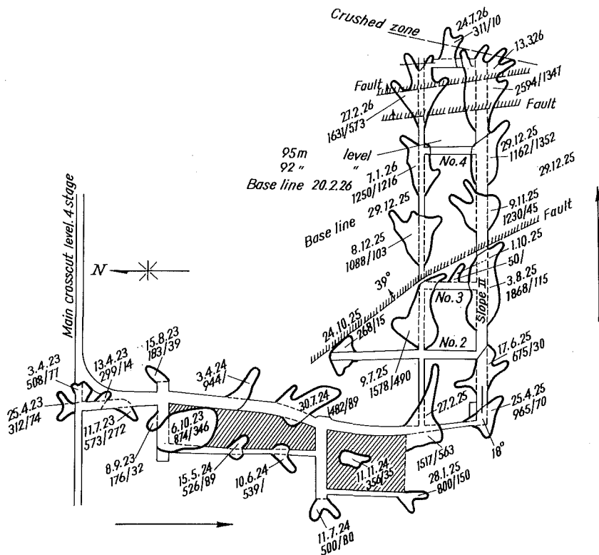
Fig. 2.5) Outbursts of \text{CO}_2 in the Anton Seam, Ruben Colliery (by Wilson)
