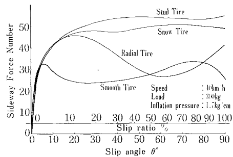
Fig. 18 Slip number and sideways force number
