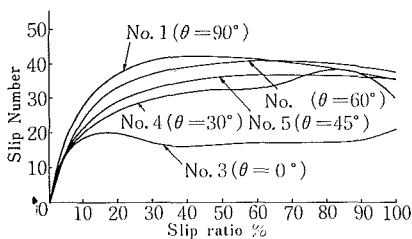
Fig. 19 Slip number and tread pattern angle
