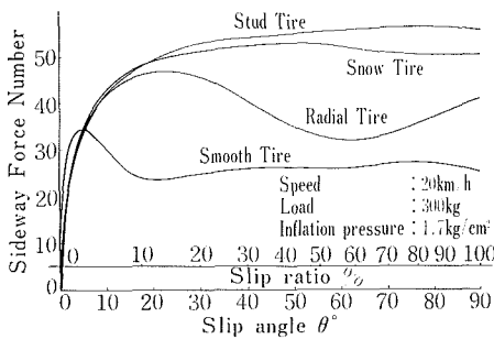
Fig. 17 Slip number and sideways force number
