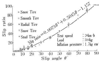
Fig. 15 Relation between slip angle and slip ratio on snow covered road surface
