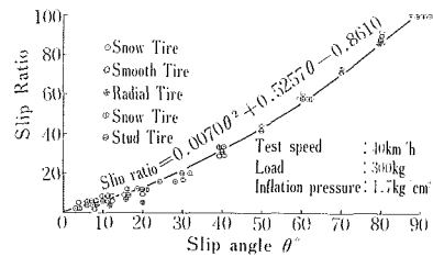
Fig. 16 Relation between slip angle and slip ratio on snow covered road surface
