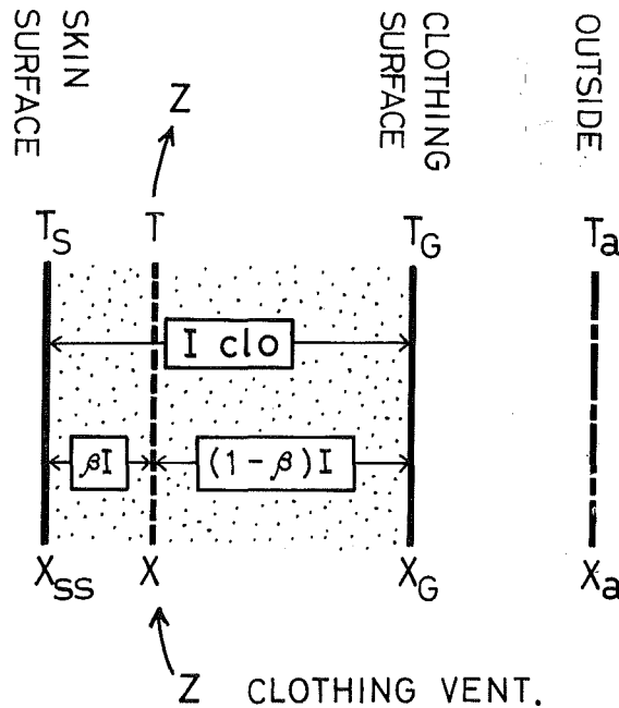
Fig. 2 Model of clothed state ( T_s - X_{ss} model)
