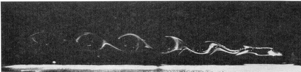
Fig. 2. Vortex pattern behind a circular cylinder in a laminar boundary layer along a flat plate (flow from right to left). Flow visualization by electrolytic dye production. Gd/U_0 = 0.49 , U_0 d/\nu = 52 ; d = diameter of cylinder (3.2 mm), U_0 = undisturbed velocity at the center of cylinder (2.5 cm/s), \nu = kinematic viscosity; boundary layer thickness \delta = 13.4 mm, normal distance between the center of cylinder and the plane wall = 0.4 \delta .
