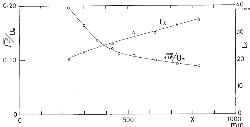
Fig. 2. Variation of intensity and scale of streamwise component of turbulence along center-line of working section.
